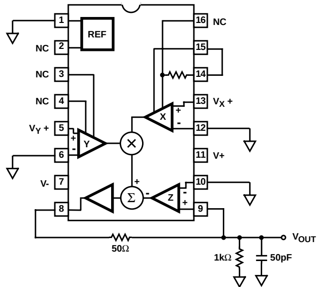
FIGURE 1. LARGE AND SMALL SIGNAL RESPONSE TEST CIRCUIT
