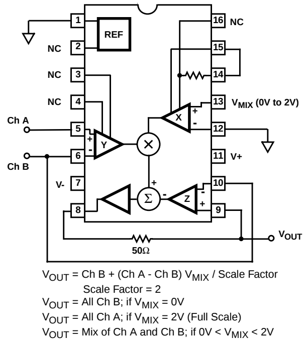
FIGURE 6. VIDEO FADER
