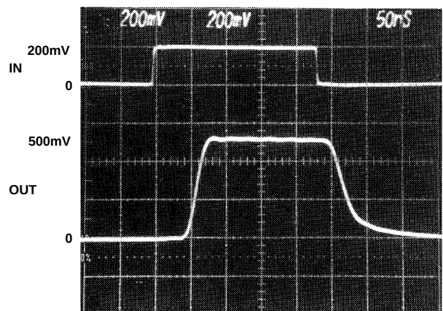
V X SMALL SIGNAL RESPONSE
