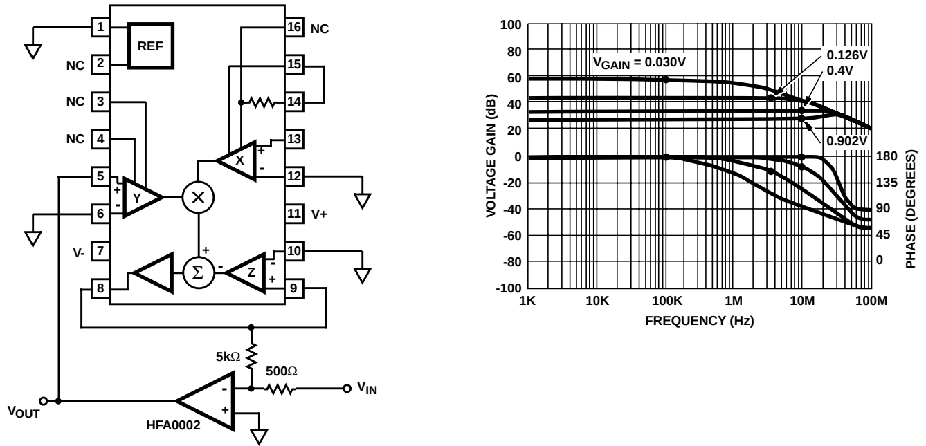
FIGURE 5. VOLTAGE CONTROLLED AMPLIFIER
