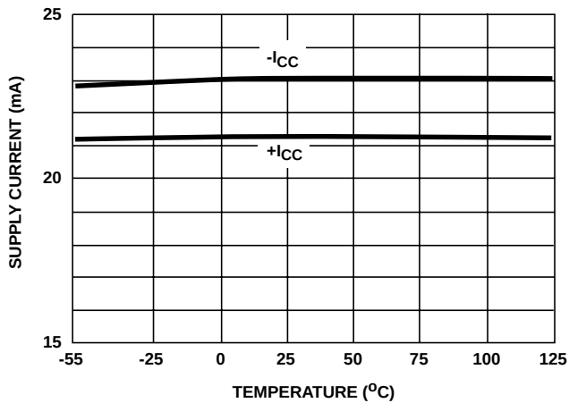
FIGURE 21. SUPPLY CURRENT vs TEMPERATURE
