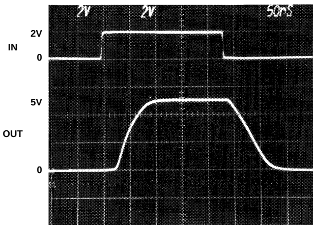
V X LARGE SIGNAL RESPONSE
